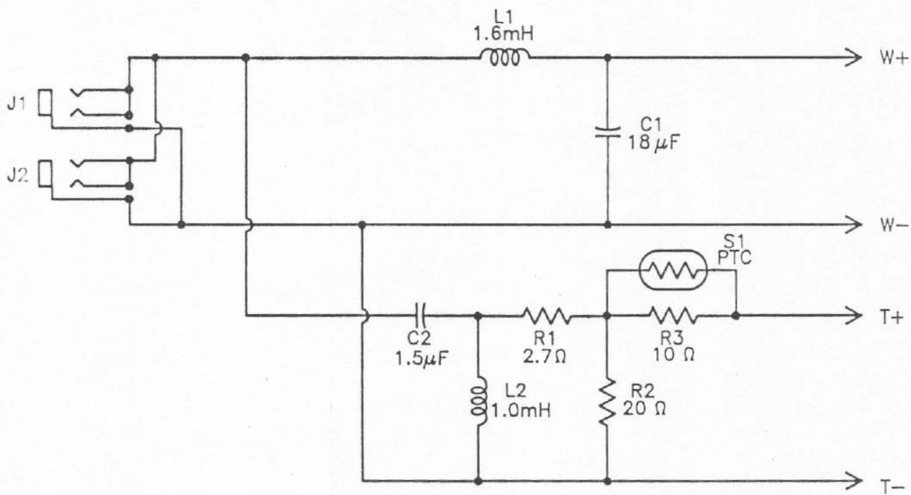
SCHEMATIC DIAGRAM
