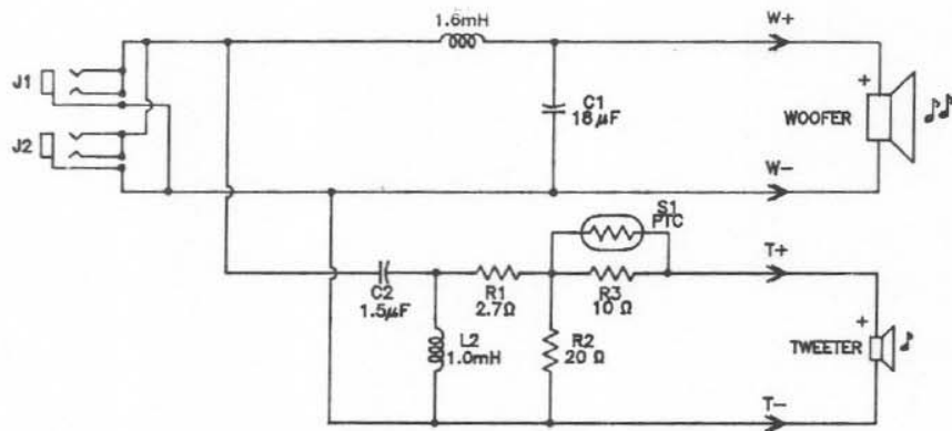
SCHEMATIC DIAGRAM
